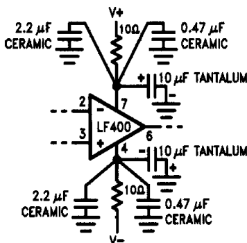
FIGURE 2. Power Supply Bypassing (see Text)
