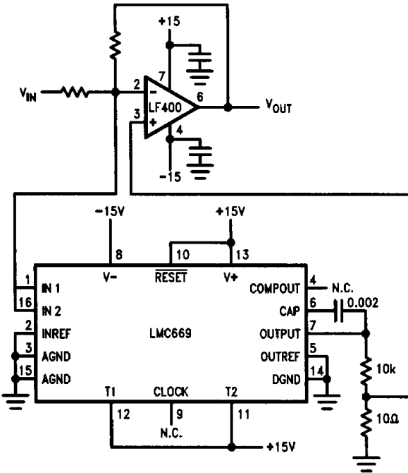
FIGURE 4b. Automatic Offset Adjustment Using LMC669
